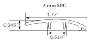
SURFACE REDUCER
